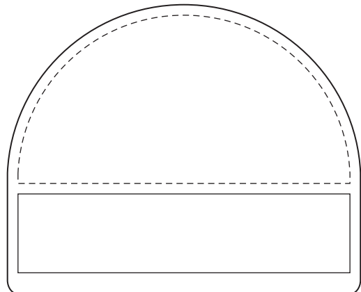
31-5600 size 67x55, printed area 63x32
