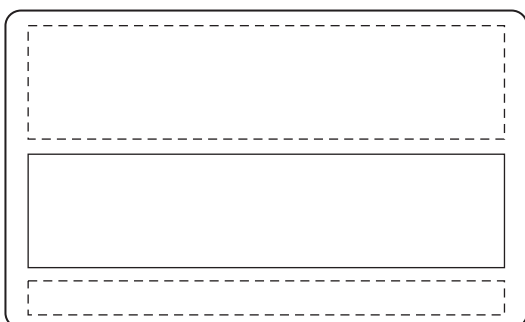
31-5900 size 69x42, printed area 63x15 (4,5)
