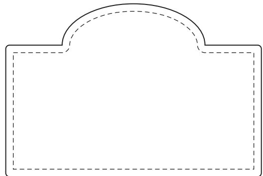
31-2708 size 68x46, printed area 64x42
