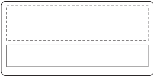
31-5200 size 70x34 printed area 65x16
